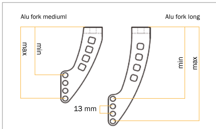
Aluminium caster fork (AF), Seat height front (without seat inclination)
